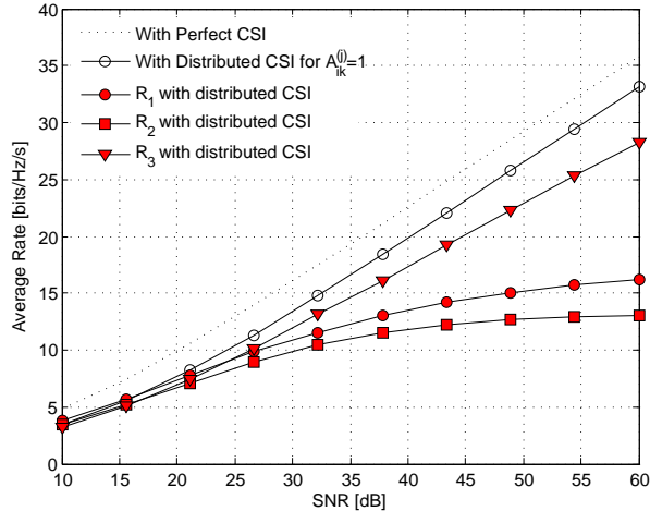
Fig. 1: Average rate per user in the square setting M = N = 4 with d = 2 for the CSIT scaling coefficients given in (35).
