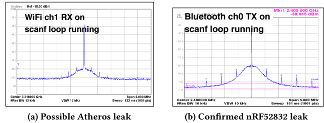
Figure 13: A possible screaming channel carrier on a Qualcomm Atheros AR9721, with spurs which change depending on the code being executed. Besides, a confirmed leak on the nRF52832 .
