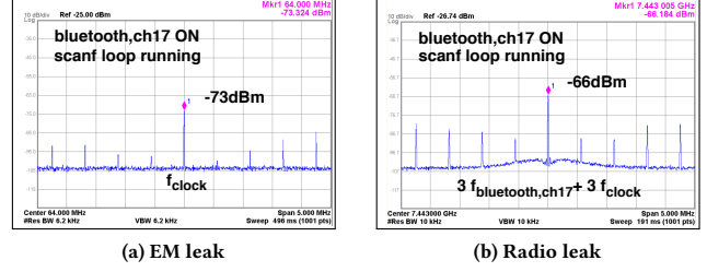
Figure 12: Leaks resulting from executing printf on a Nordic Semiconductor nRF52840. Note the central frequency is 64 MHz in (a) and of 7.443 GHz in (b).
