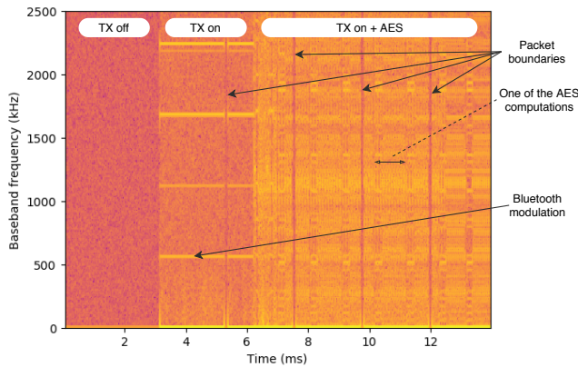
Figure 3: Spectrogram of the radio emissions from a Nordic Semiconductor nRF52832 over time, captured at 2.528 GHz with Ettus Research USRP B200 mini via cable, sampling at 5 MHz (brighter colors indicate higher signal amplitude).
