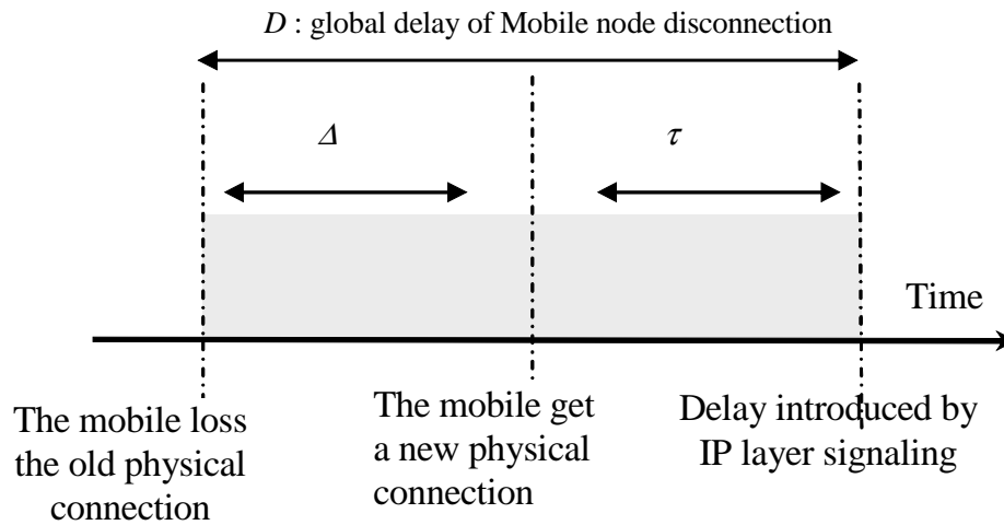
Figure III-1 IP handover delay
