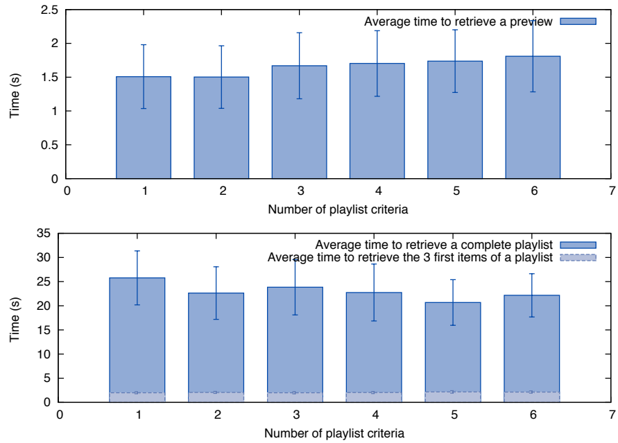
Fig. 6. Response time for the preview and the playlist over 600 user queries
