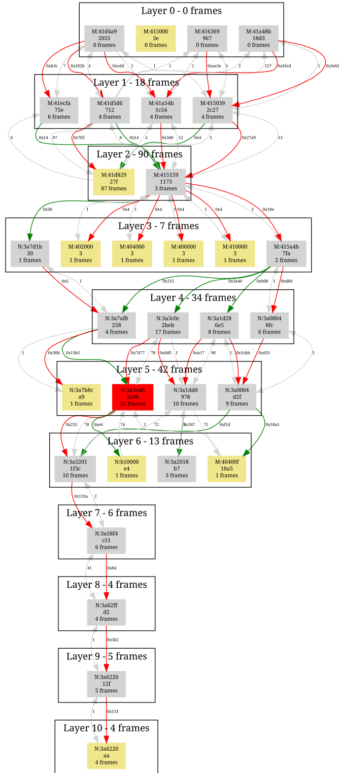
Fig. 3. Graph generated for Obsidium 1.2, a Type-IV packer with several threads, interleaved execution, and a multi-frame unpacking routine. The original code, located at layer \mathcal{L}_6 , starts at address 0x0040400f , is 0x18a5 bytes long and is unpacked in one single frame (i.e., it is fully unpacked before being executed). The last executed instructions belong to the unpacking routine (red node at layer \mathcal{L}_5 ).
