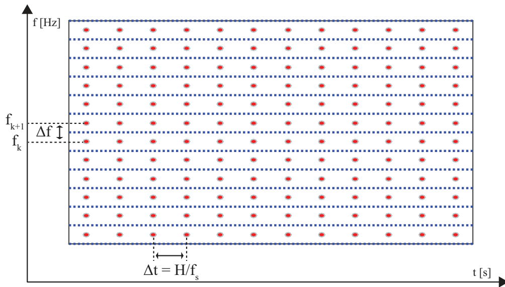
(a) FFT
